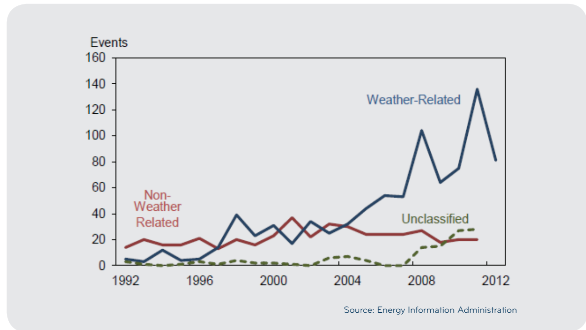
Categorised outages in the American electricity system Observed Outages to the Bulk Electric System, 1992-2012
