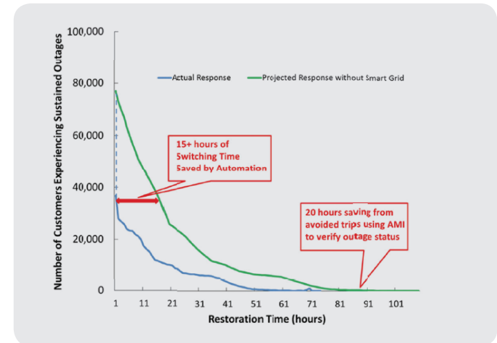
Figure M: Automation has greatly reduced the number of customer-hours of outage experienced
